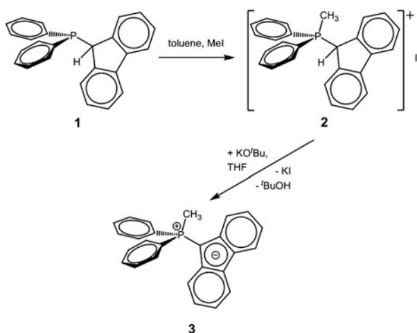
Scheme 1. Synthesis of the phosphonium ylide 3.
