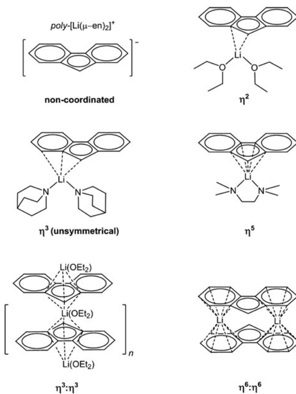
Chart 1. Observed coordination modes of the fluorenyl anion in its lithium complexes.
