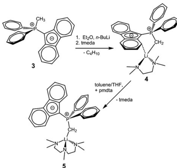
Scheme 2. Synthesis of lithium derivatives 4 and 5.
